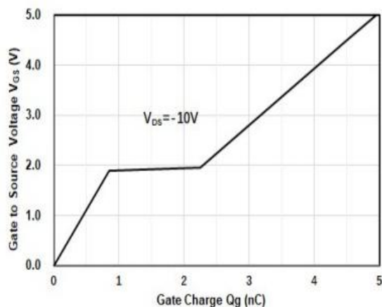
Figure 6: Gate-Charge Characteristics
