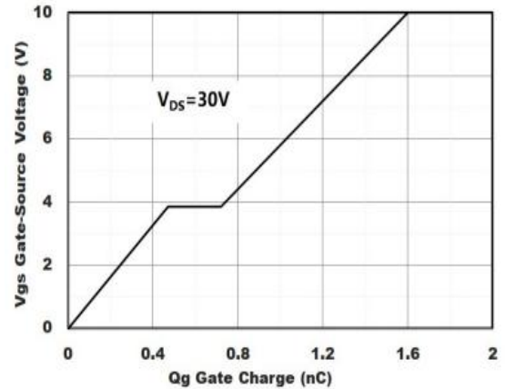
Figure 6: Gate-Charge Characteristics
