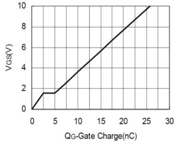
Figure 6: Gate-Charge Characteristics
