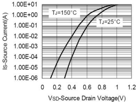
Figure 9: Diode Characteristics
