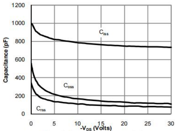
Figure 5: Capacitance Characteristics
