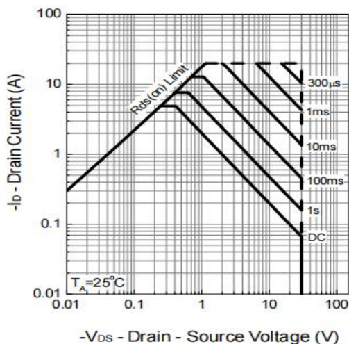
Figure 10: Safe Operating Area
