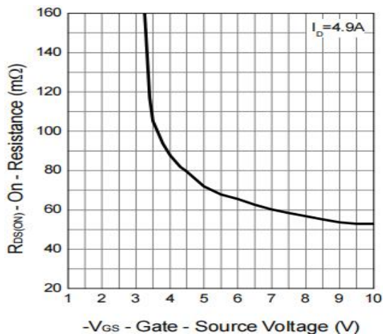
Figure 8: On-Resistance vs. V_{GS}
