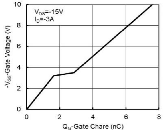
Figure 6: Gate-Charge Characteristics
