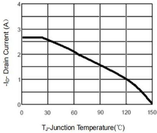
Figure 7: Drain Current vs. Temperature
