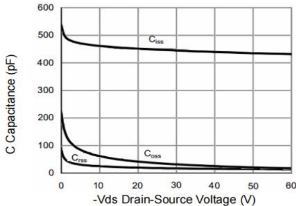
Figure 5: Capacitance Characteristics
