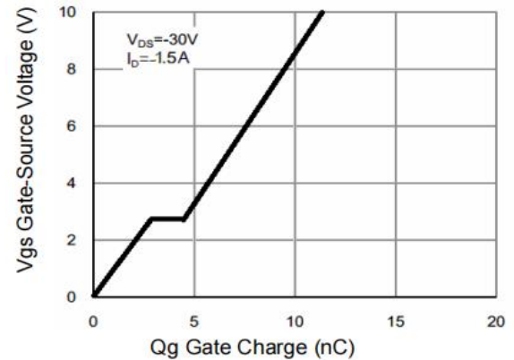
Figure 6: Gate-Charge Characteristics
