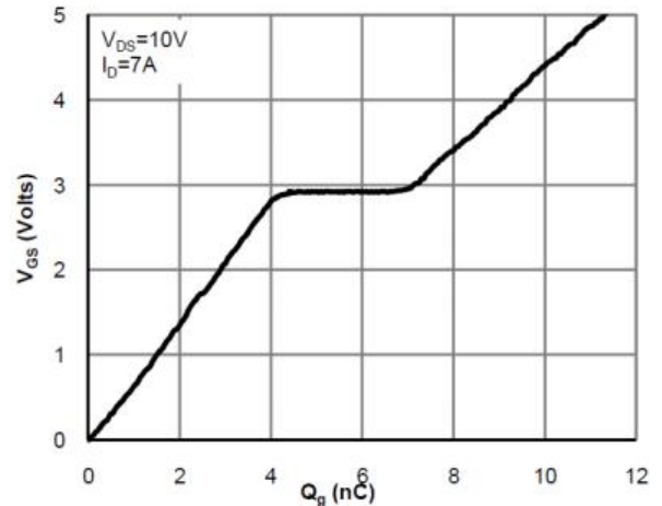
Figure 6: Gate-Charge Characteristics
