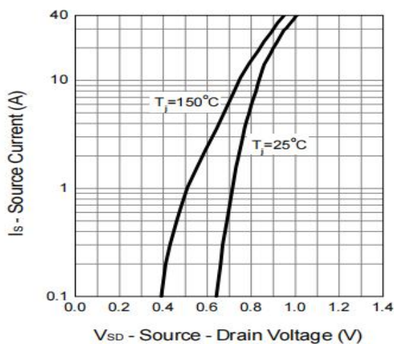
Figure 9: Diode Characteristics
