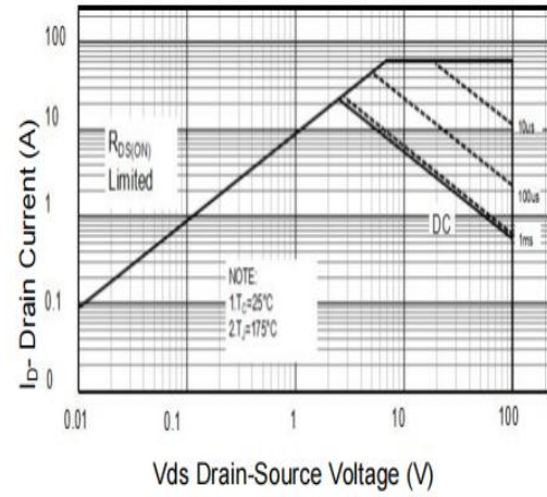
Figure 4: Safe Operating Area
