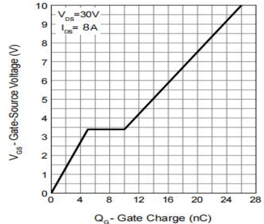
Figure 6: Gate-Charge Characteristics
