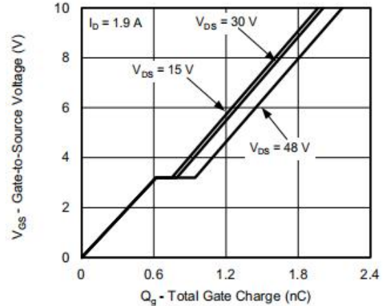
Figure 6: Gate-Charge Characteristics
