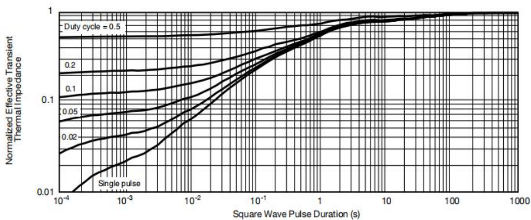
Figure 9: Transient Thermal Response Curve
