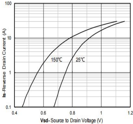
Figure 9: Diode Characteristics
