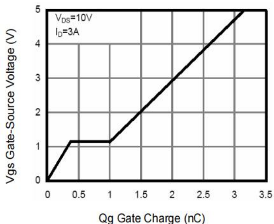
Figure 6: Gate-Charge Characteristics
