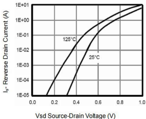
Figure 9: Diode Characteristics
