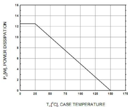
Figure 6. Power Derating
