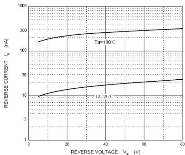
Figure 2: Leakage Current
