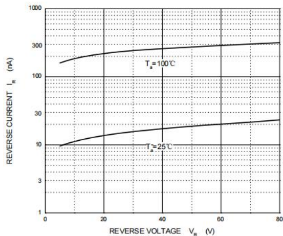
Figure 2: Leakage Current
