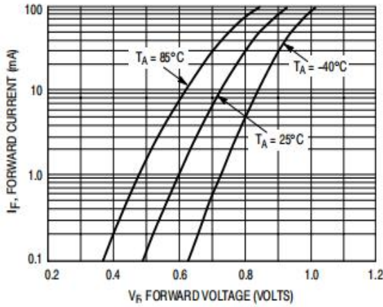
Figure 1: Forward Characteristics
