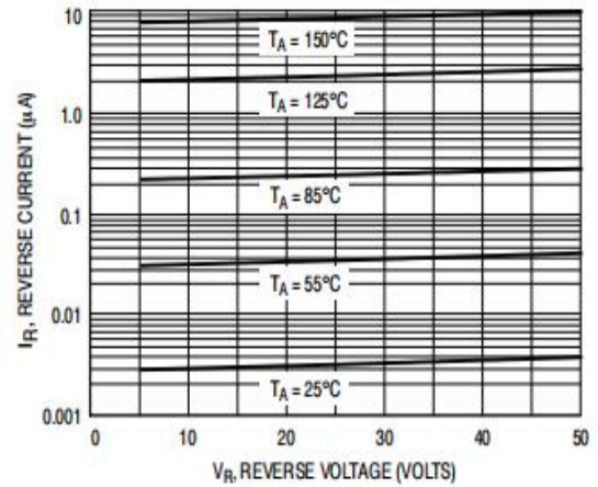
Figure 2: Leakage Current
