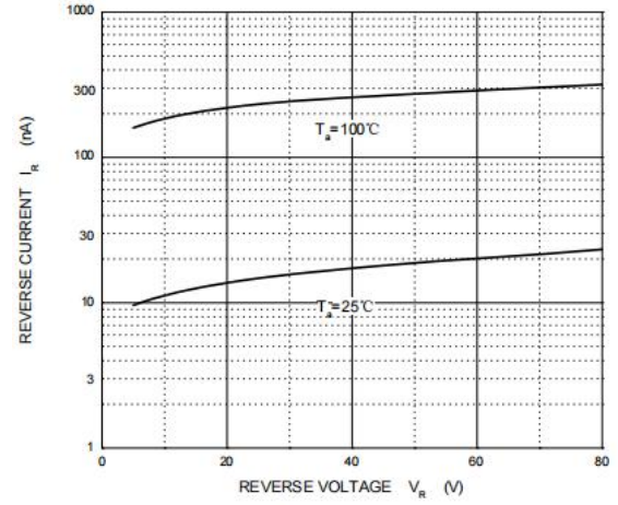
Figure 2: Leakage Current
