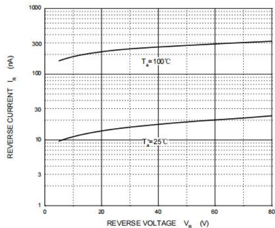
Figure 2: Leakage Current
