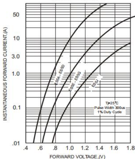
FIG.3-TYPICAL FORWARD CHARACTERISTICS
