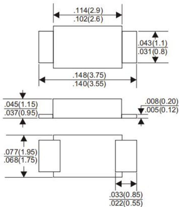
SOD-123FL
