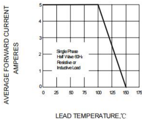
FIG.3 -- FORWARD DERATING CURVE
