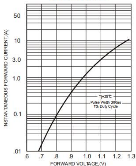
FIG.1-TYPICAL FORWARD CHARACTERISTICS
