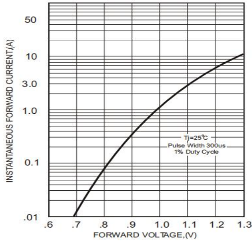
Figure 1: Forward Characteristics
