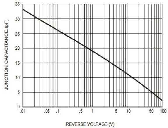
Figure 4: Junction Capacitance
