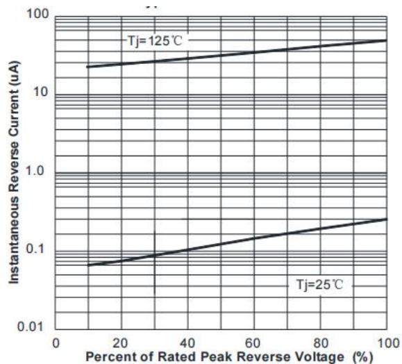
Figure 4: Reverse Leakage Characteristics
