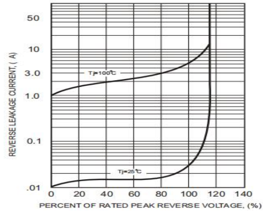
Figure 4: Reverse Leakage Characteristics
