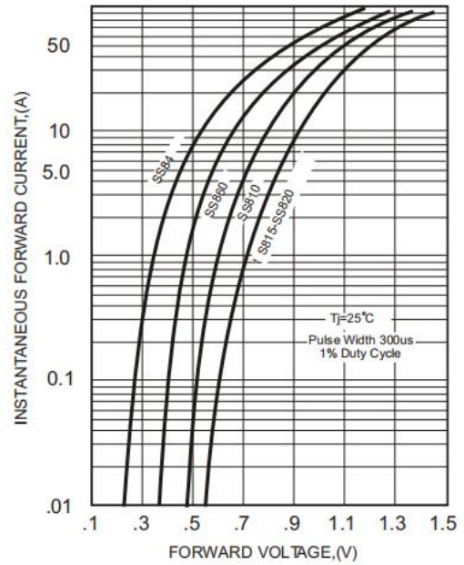
FIG.2-TYPICAL FORWARD CHARACTERISTICS
