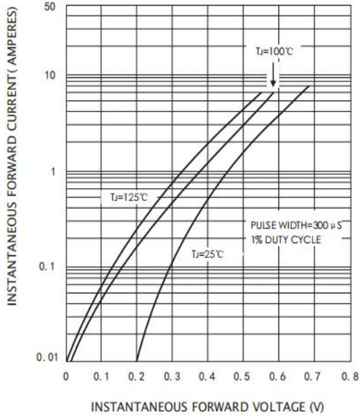
Figure 3: Forward Characteristics
