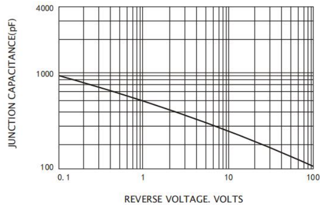
Figure 5: Capacitance Characteristics
