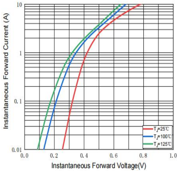
Figure 3: Forward Characteristics
