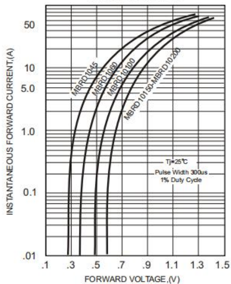
FIG.2-TYPICAL FORWARD CHARACTERISTICS
