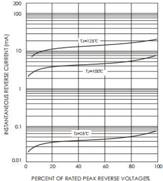
Figure 4: Reverse Characteristics
