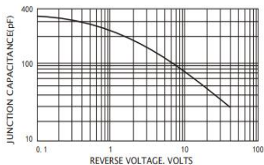
Figure 5: Capacitance Characteristics
