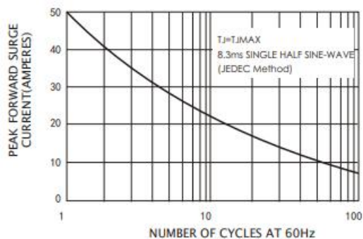
Figure 2: Forward Surge Current Curve
