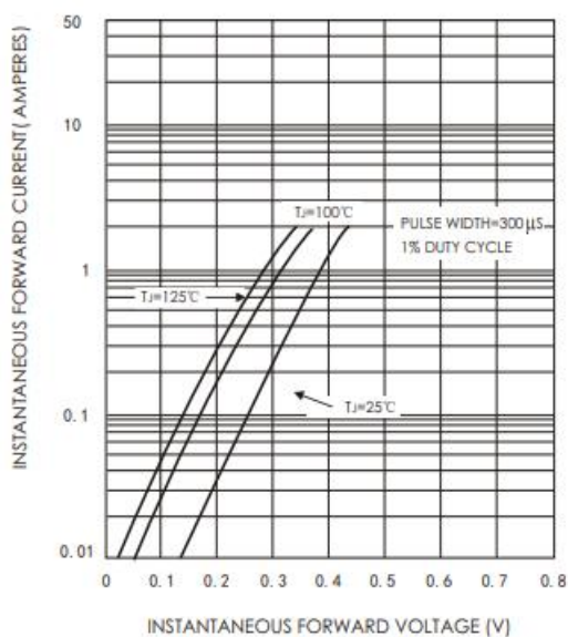
Figure 3: Forward Characteristics
