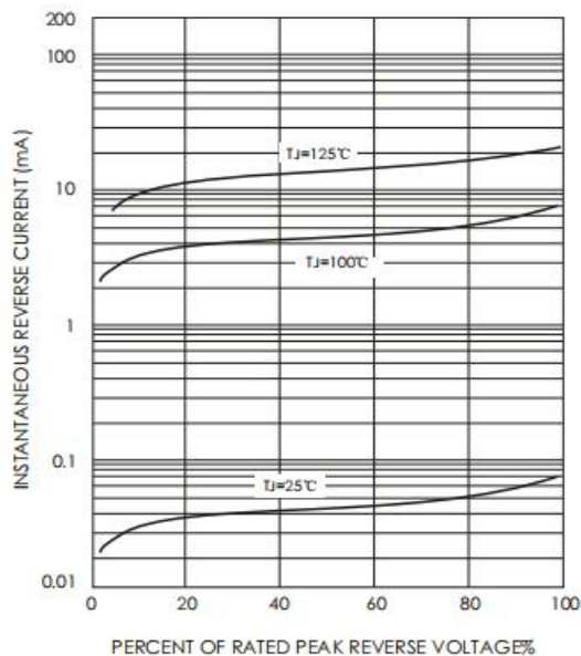
Figure 4: Reverse Characteristics
