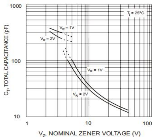
Figure 4: Capacitance Characteristics
