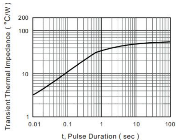
Figure 2: Zener Impedance Characteristics
