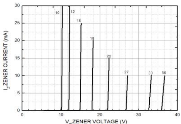
Figure 1: Zener Characteristics
