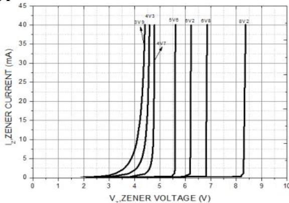
Figure 1: Zener Characteristics
