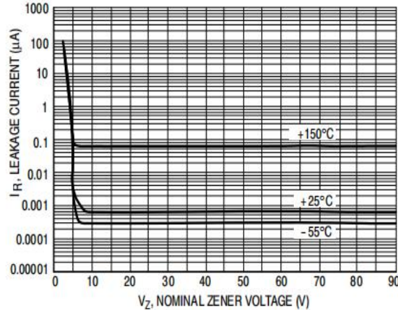
Figure 5: Leakage Current
