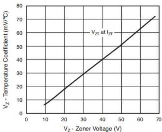
Figure 5: Temperature Coefficient
