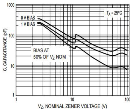
Figure 4: Capacitance Characteristics
