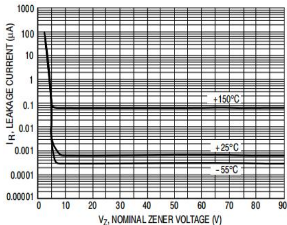
Figure 5: Leakage Current
