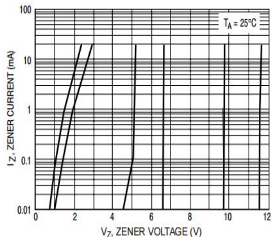
Figure 2: Zener Breakdown Characteristics
