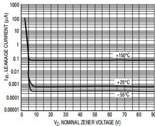
Figure 6: Leakage Current
