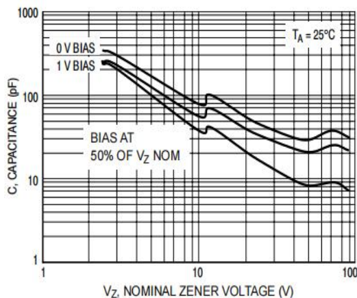
Figure 4: Capacitance Characteristics
