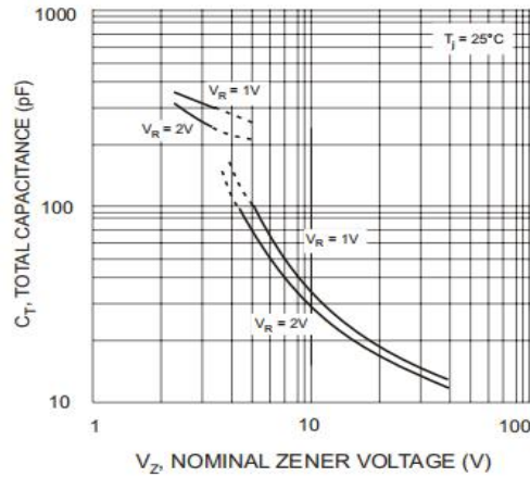
Figure 2: Capacitance Characteristics
