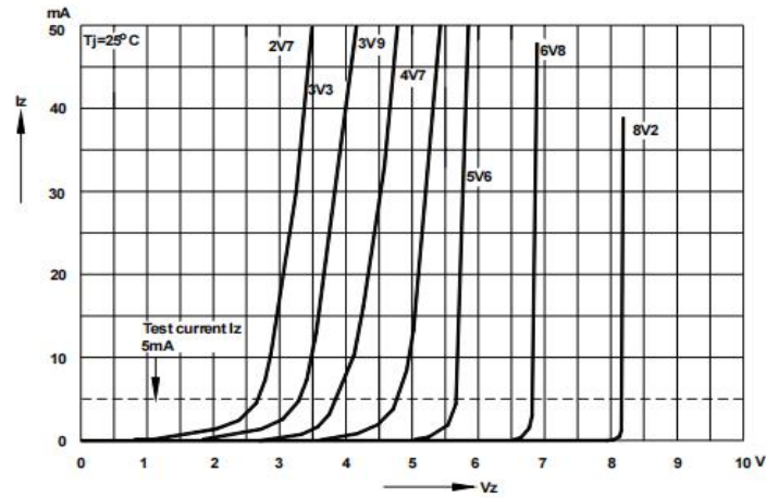
Breakdown characteristics T_j = \text{constant (pulsed)}
