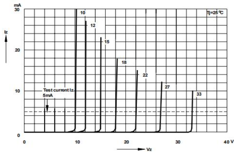
Breakdown characteristics T_j = \text{constant (pulsed)}
