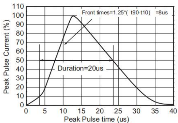
8/20us waveform
