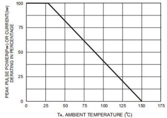
FIG.2-PULSE DERATING CURVE
