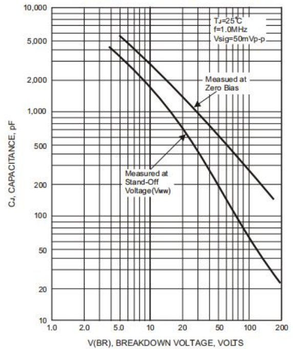
FIG.4-TYPICAL JUNCTION CAPACITANCE
