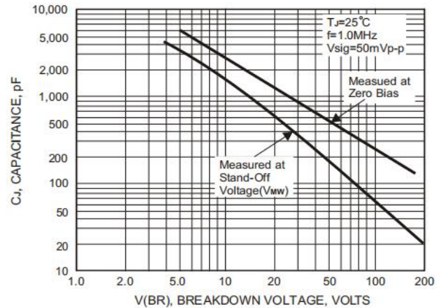
Figure 4: Junction Capacitance
