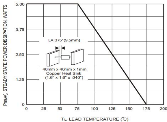
Figure 5: Power Derating
