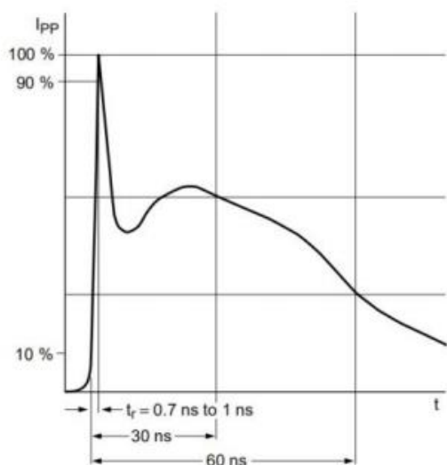
IEC61000-4-2 Waveform
