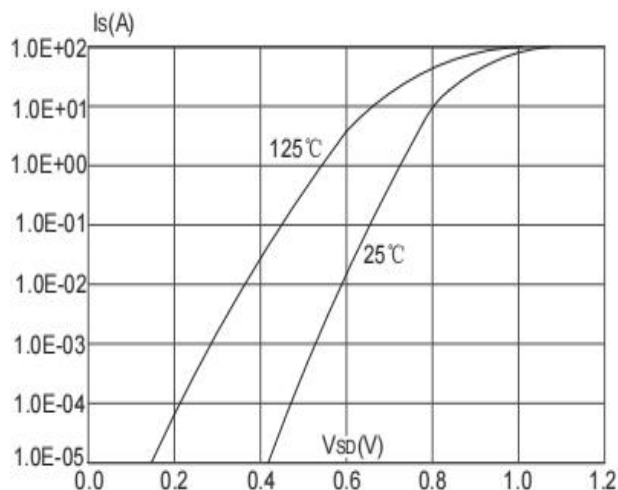
Figure 9: Diode Characteristics
