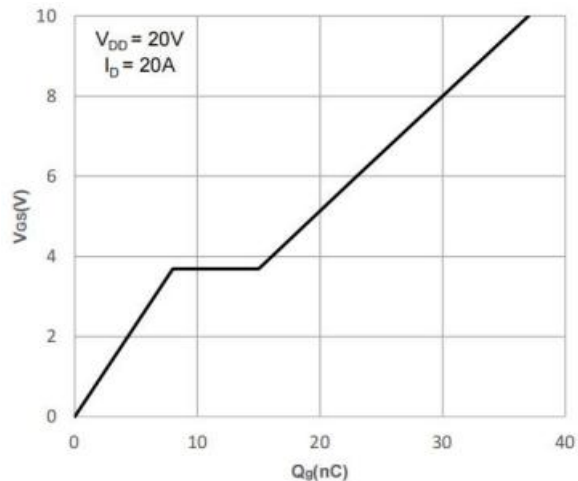
Figure 6: Gate-Charge Characteristics
