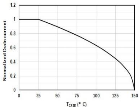
Figure 8: Drain Current vs. T_C
