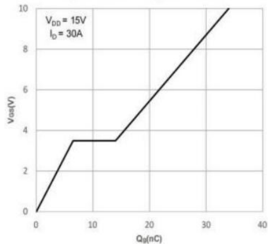
Figure 6: Gate-Charge Characteristics
