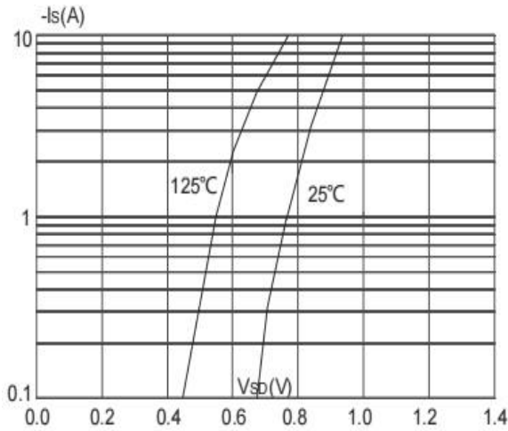
Figure 7: Diode Characteristics
