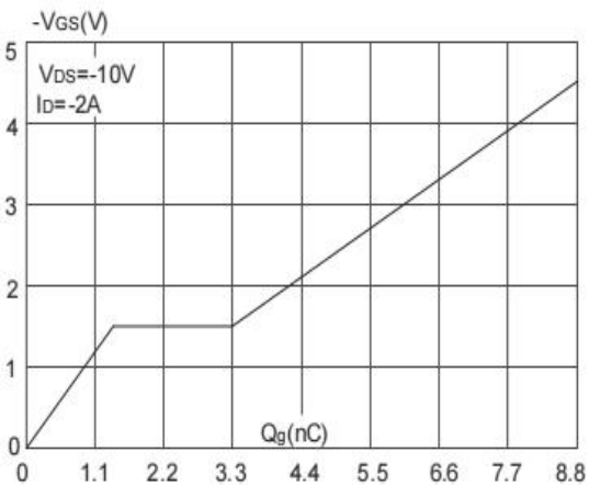
Figure 6: Gate-Charge Characteristics
